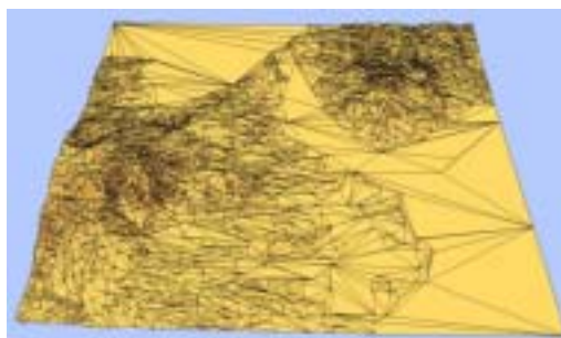
M^{5152} with 1988 triangles.
