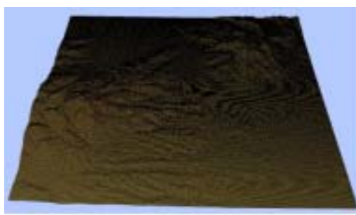
M^{103037} with 204800 triangles.
