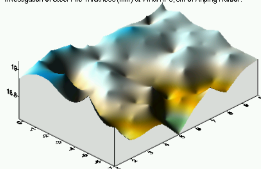
Investigation of Steel Pile Thickness (mm) at Wharf# 3, 0m of Anping Harbor.
